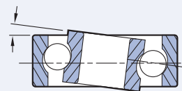
Figure 5. Free angle of the bearing.
