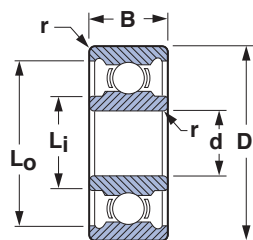
OPEN BEARING
