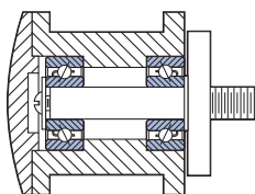
Figure 3. Typical Tape Guide design using screw and washer to solidly preload by clamping inner rings – Outer Ring Rotation
